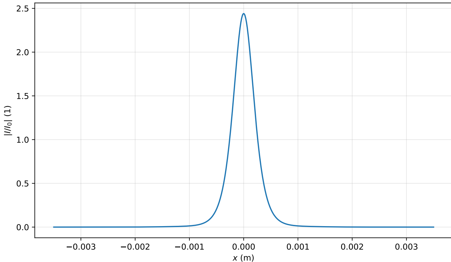
Intensity profile I(x, y = 0, z = 2.627m)/I_0 , P_{in}=1.0P_{cr} , artificial time
